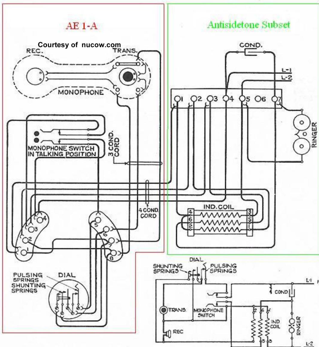
Circuit H-17824
